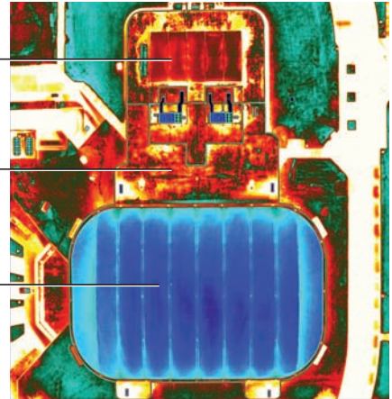
New traditional built-up roof
